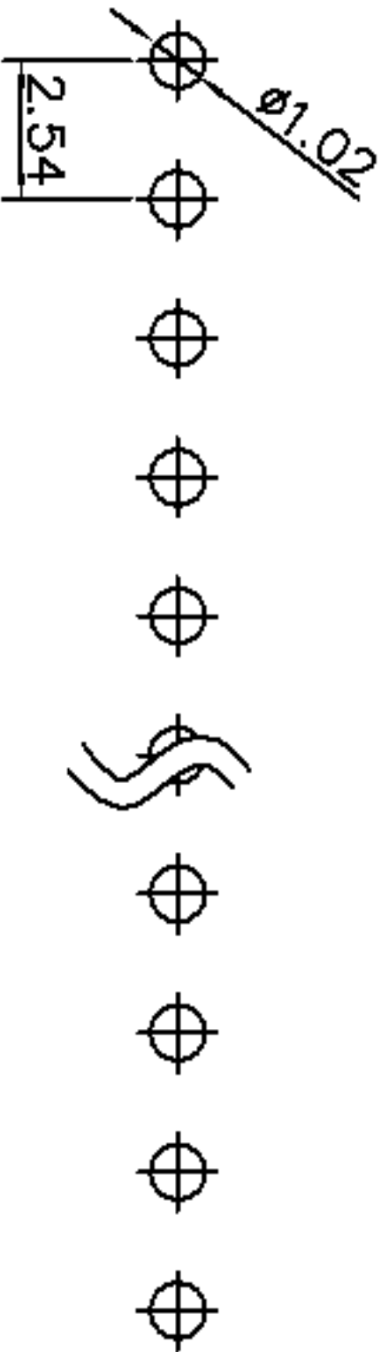
PCB Layout
